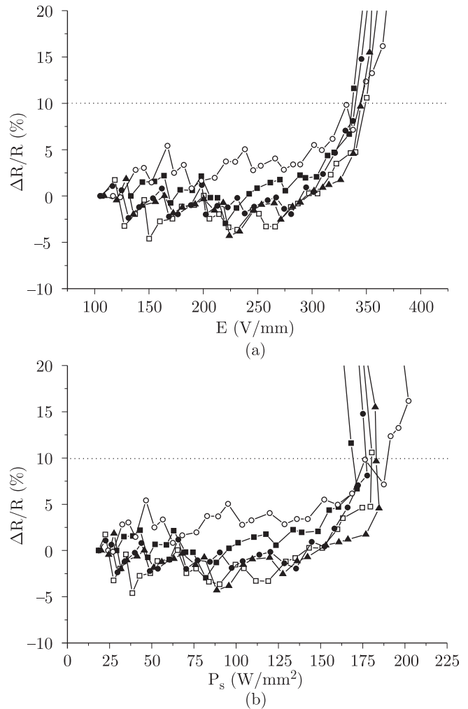
Fig. 10. Relative resistance changes versus electric field and pulse surface power density for 200 \times 200 \text{ }\mu\text{m}^2 thick-film microresistors screen-printed on alumina ( t_p = 0.1 \text{ ms} )
