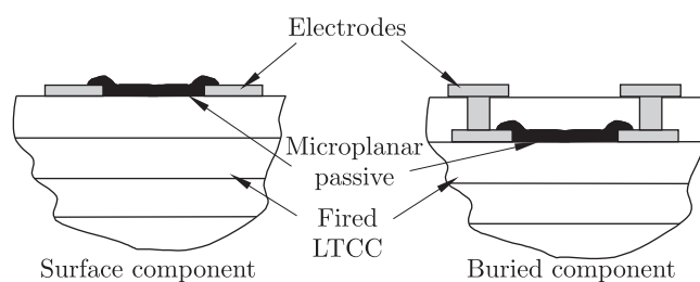
Fig. 2. Schematic cross-section of surface and buried microplanar microelectronic resistor
