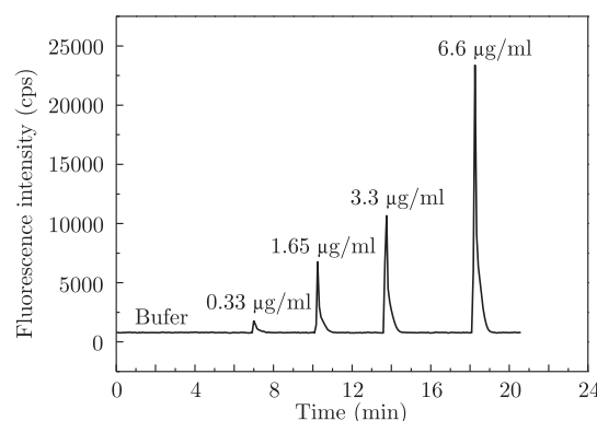
Fig. 4. Fluorescence signal versus time for different concentrations of fluorescein solution injected
