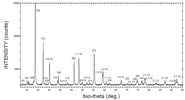
Fig. 1. The XRD pattern of BBN ceramics
