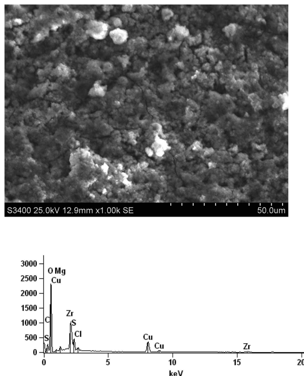
Fig. 4. SEM image and EDX spectrum of zirconium deposited on copper substrate
