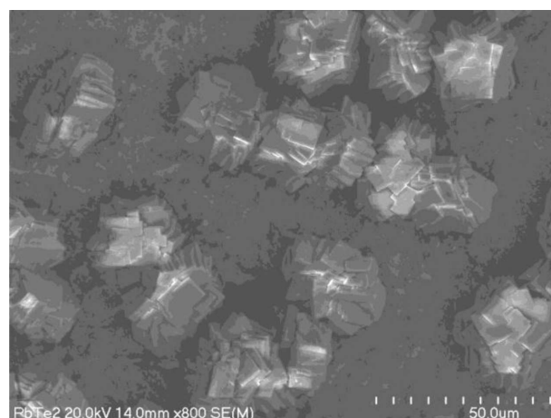
Fig. 6. Morphology of the PbTe surface anodically oxidized in HNO 3 of pH 1.5
