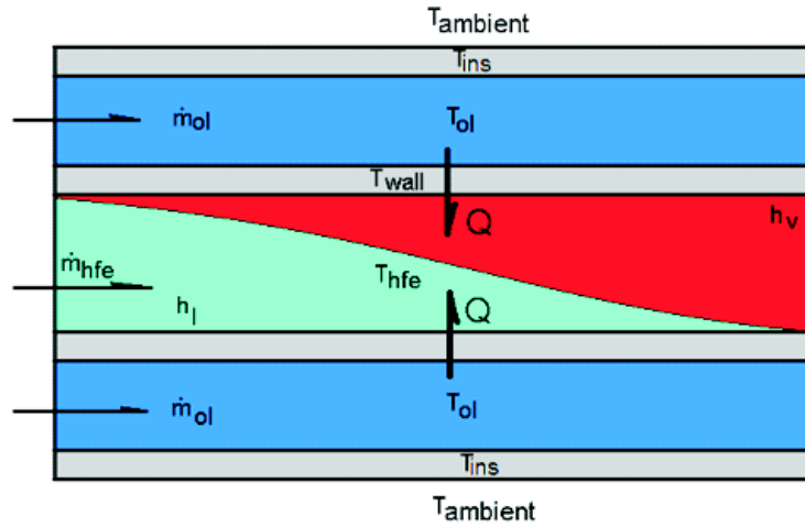
Figure 4. Graphical interpretation of the boiling process in the exemplary heat exchanger.
