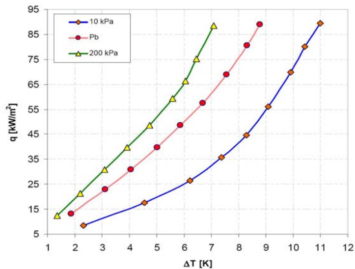
Fig. 9. Boiling curves of the smooth stainless steel tube in water- \text{Al}_2\text{O}_3 nanofluid with 0.1% concentration
