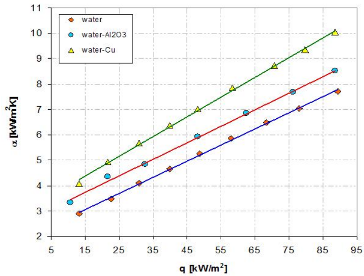
Fig. 5. Heat transfer coefficient vs. heat flux density for water- \text{Al}_2\text{O}_3 and water-Cu nanofluids of 1% concentration while boiling at 10 kPa
