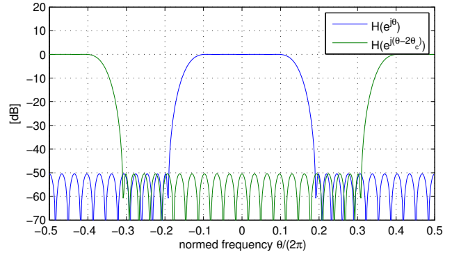
Fig. 4. Example of characteristics of H(e^{j\theta}) and H(e^{j(-\theta-2\theta_c)}) for \theta_c = 2\pi \cdot 0.25 .
