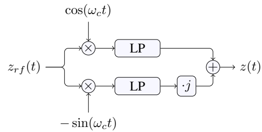
(a) quadrature demodulator in the real notation
