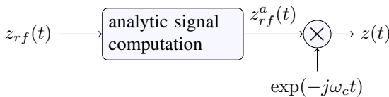
Fig. 1. Obtaining the analogue baseband signal as a demodulated analytic signal.
