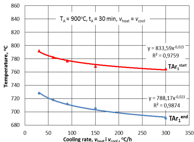
Fig. 4. The effect of cooling the tested ductile cast iron from the austenitization temperature on values of temperatures TAr_1^{start} and TAr_1^{end} after applying the heating rate equaling the cooling rate from the austenitization temperature. Austenitization temperature T_A = 900^\circ\text{C} . Austenitization time t_A = 30 min
